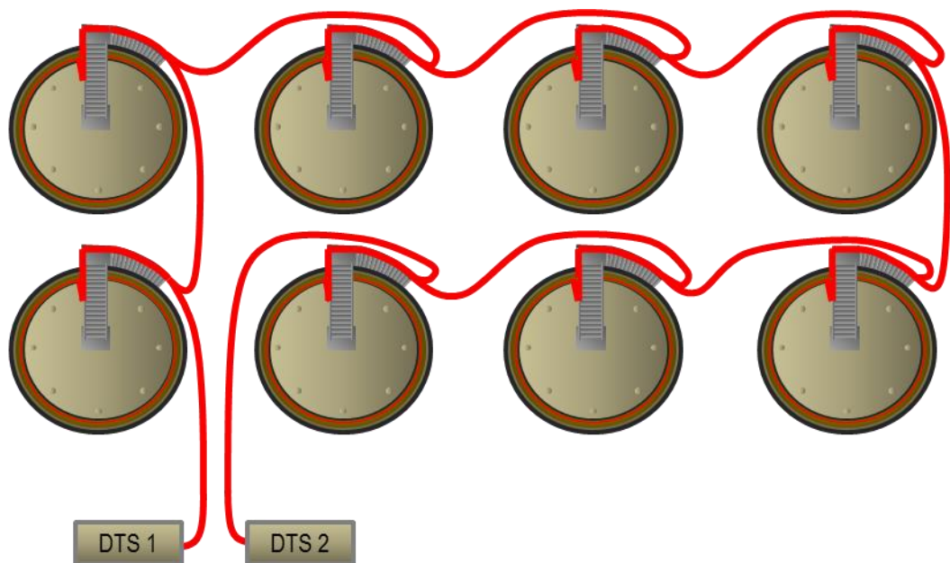
Monitoring tanks with two DTS instruments offers full redundancy
