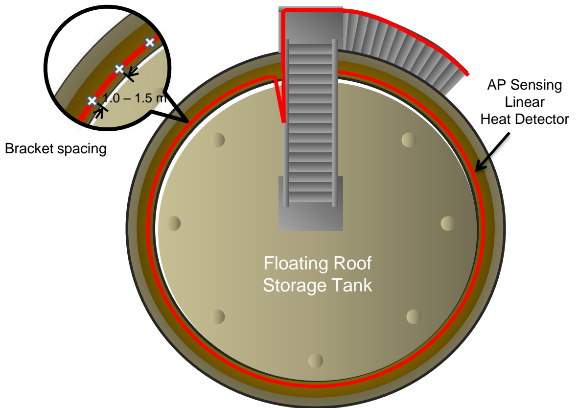
Top view – bracket spacing of sensor cable
